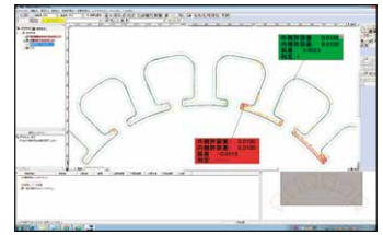
Tolerancing example
